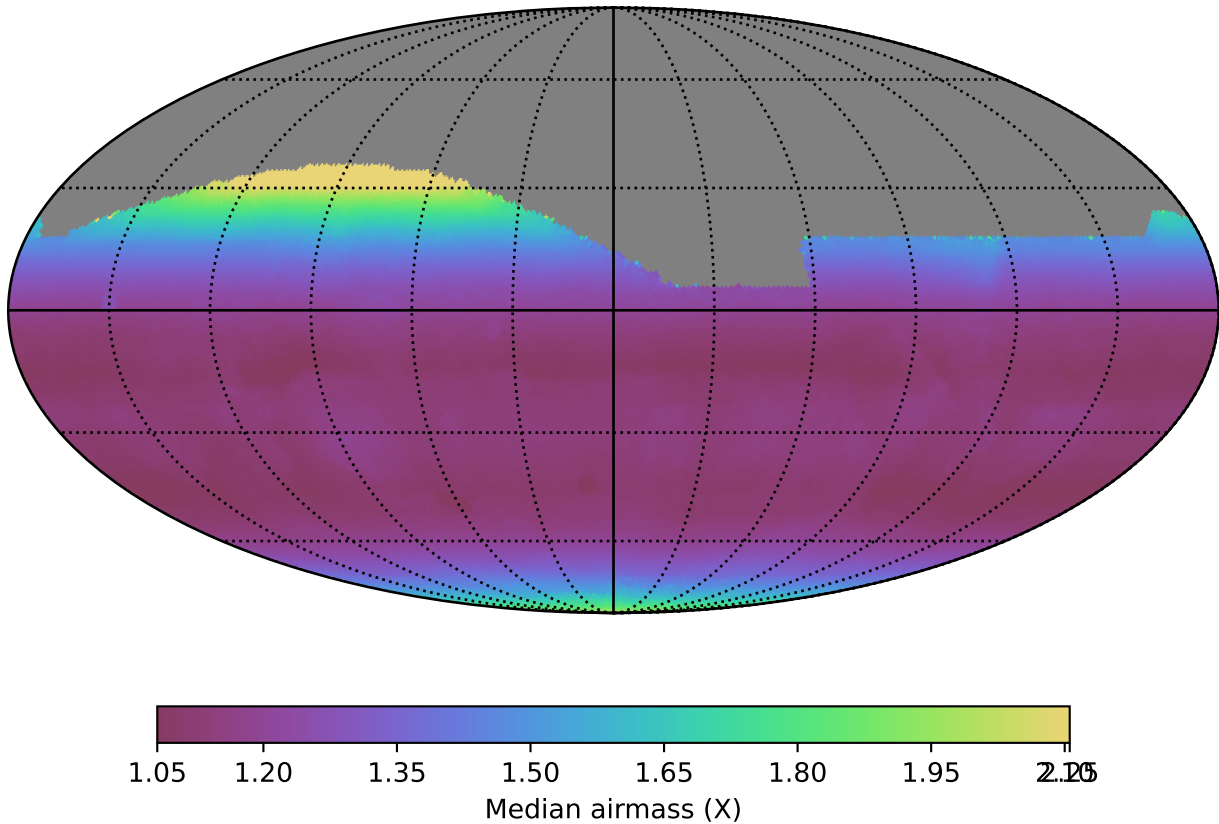
baseline_v2.1_10yrs All sky all bands: Median airmass
