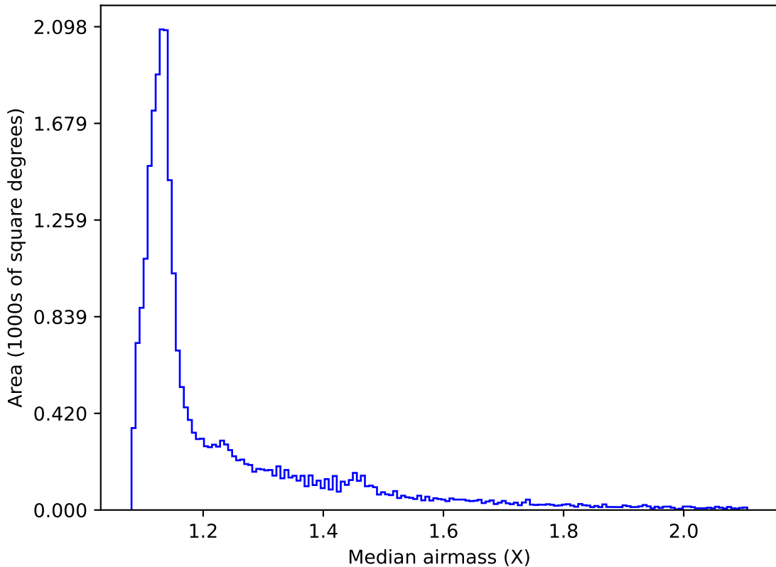
baseline_v2.1_10yrs All sky all bands: Median airmass
