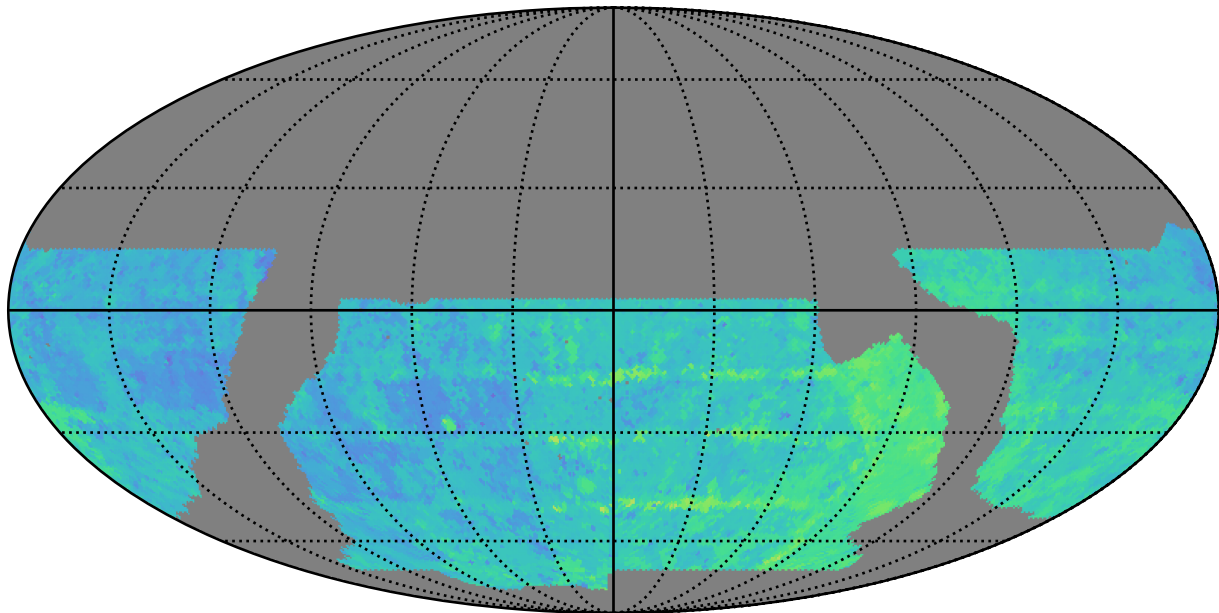
baseline_v2.1_10yrs WFD z band: Median Season Length
