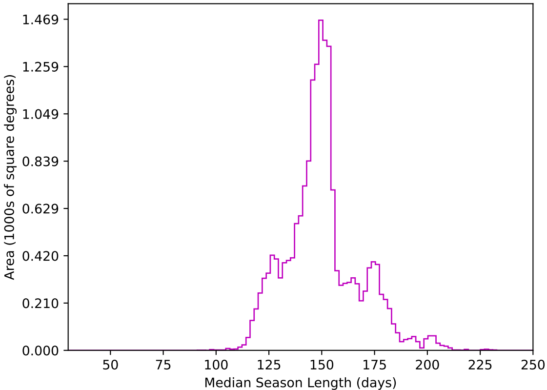
baseline_v2.1_10yrs WFD z band: Median Season Length
