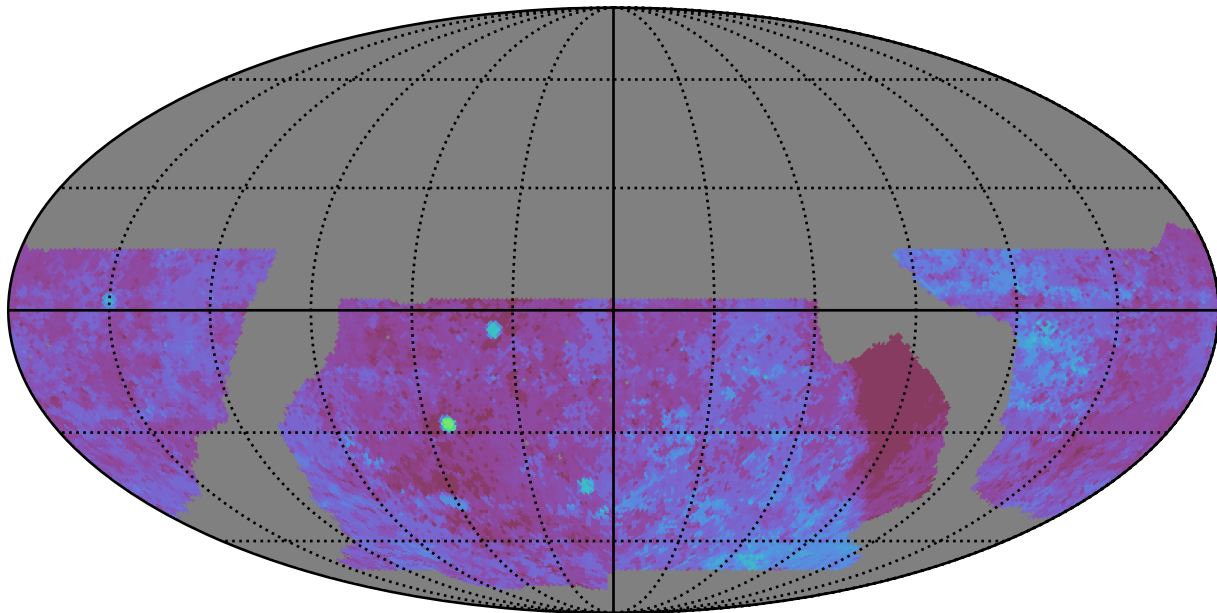
baseline_v2.1_10yrs WFD u band: Median Season Length
