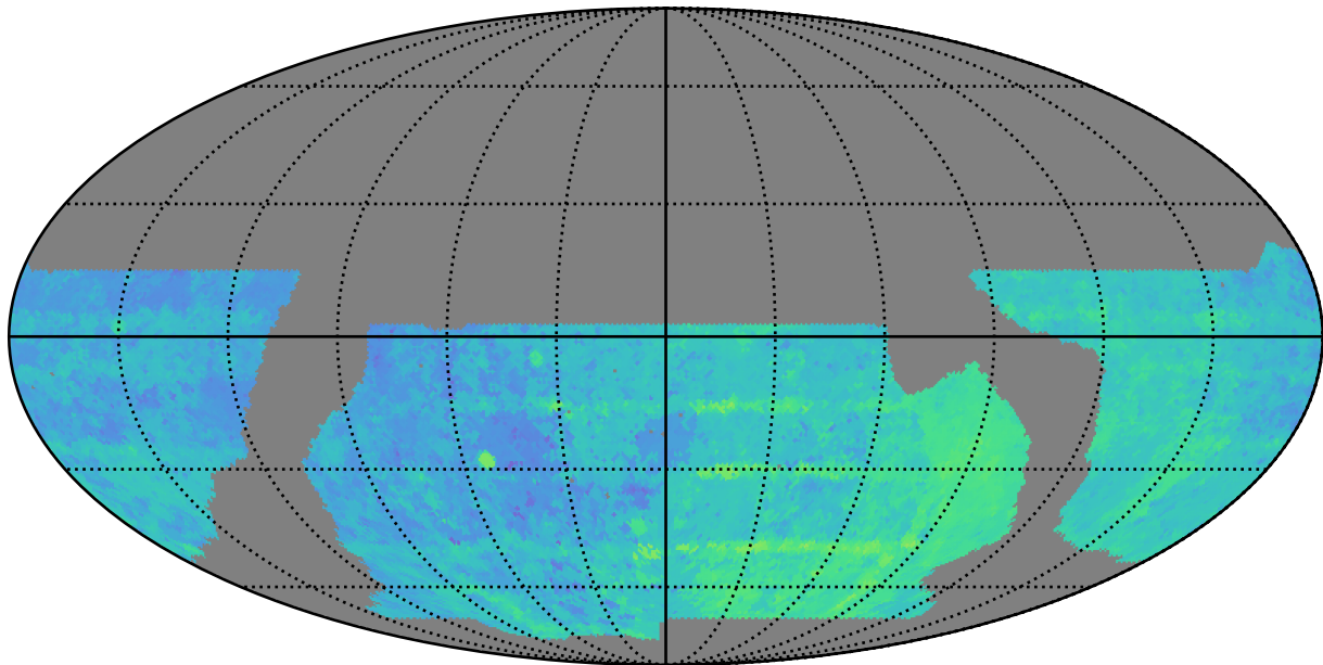
baseline_v2.1_10yrs WFD r band: Median Season Length
