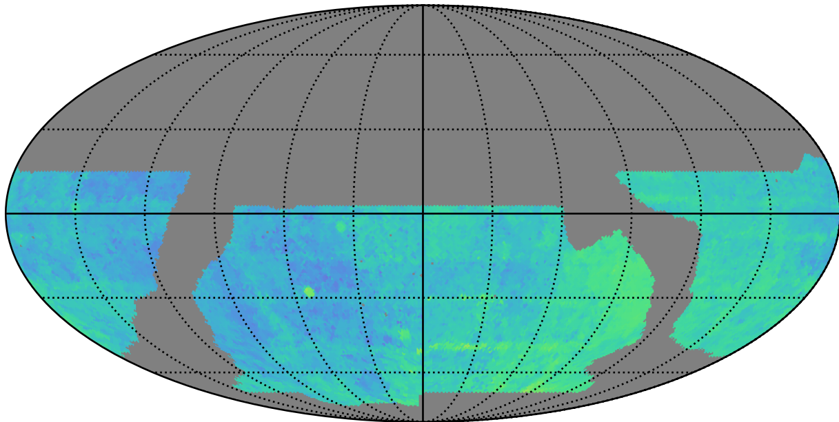
baseline_v2.1_10yrs WFD i band: Median Season Length
