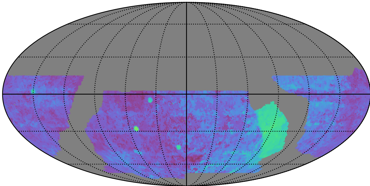
baseline_v2.1_10yrs WFD g band: Median Season Length
