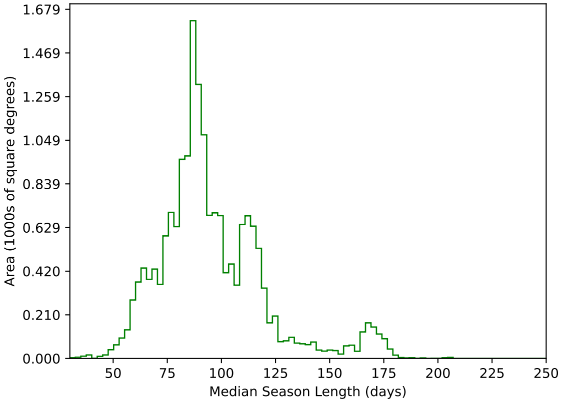
baseline_v2.1_10yrs WFD g band: Median Season Length
