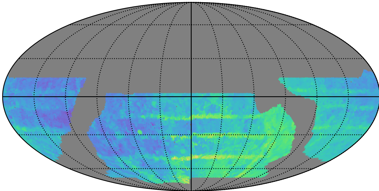
baseline_v2.1_10yrs WFD all bands: Median Season Length
