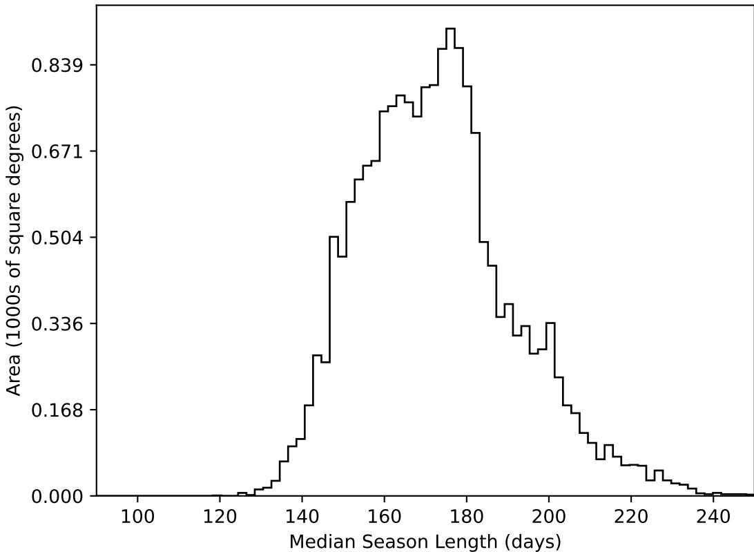
baseline_v2.1_10yrs WFD all bands: Median Season Length
