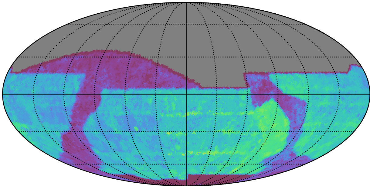
baseline_v2.1_10yrs All sky z band: Median Season Length
