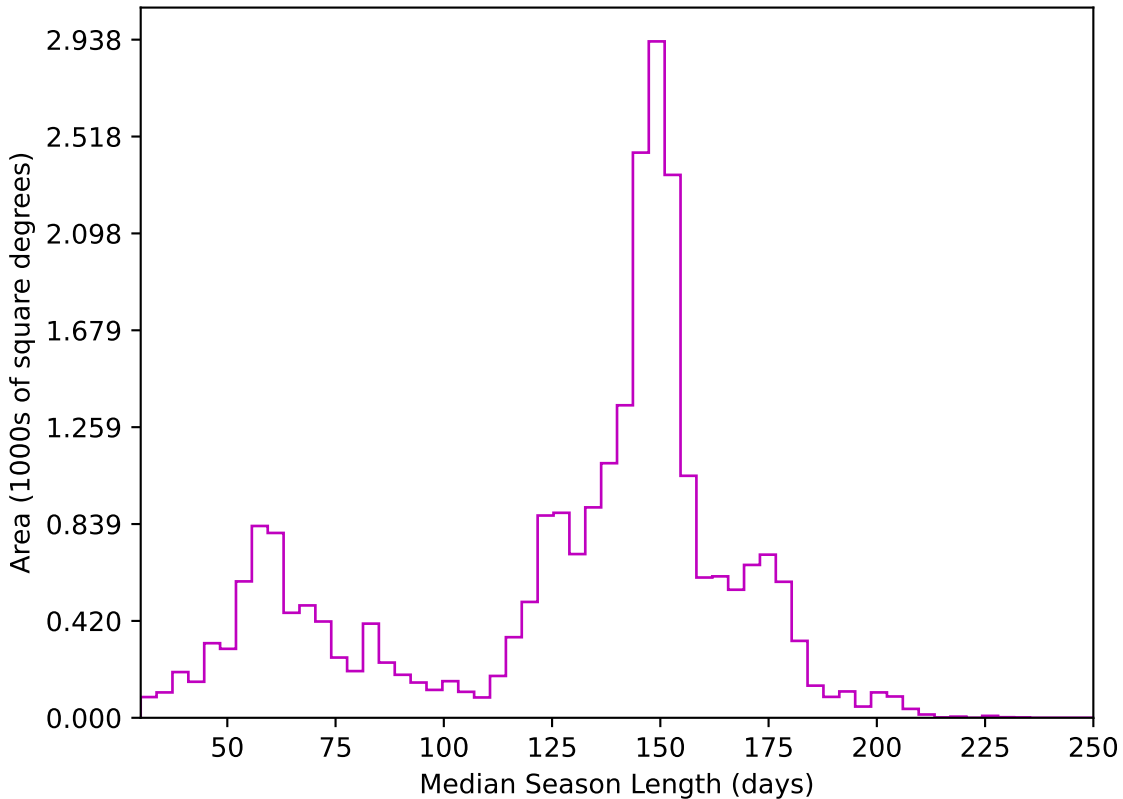
baseline_v2.1_10yrs All sky z band: Median Season Length
