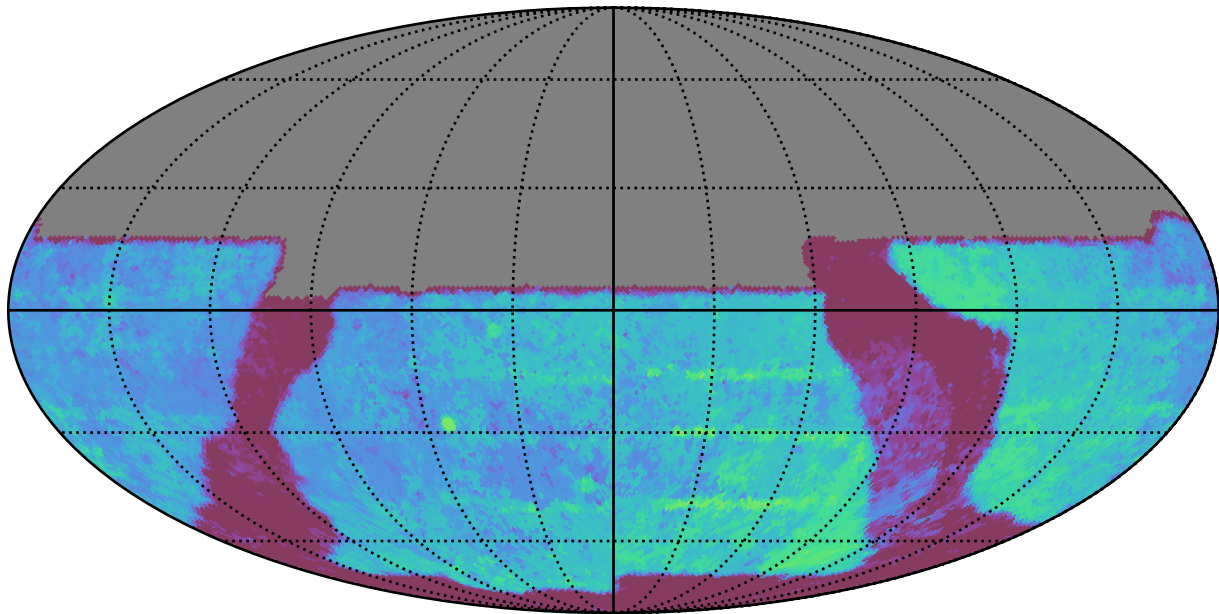
baseline_v2.1_10yrs All sky y band: Median Season Length
