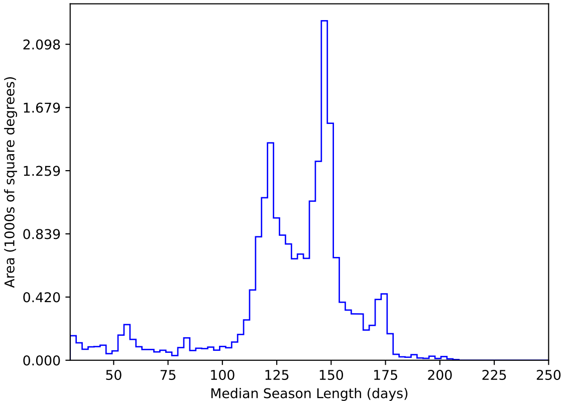
baseline_v2.1_10yrs All sky y band: Median Season Length
