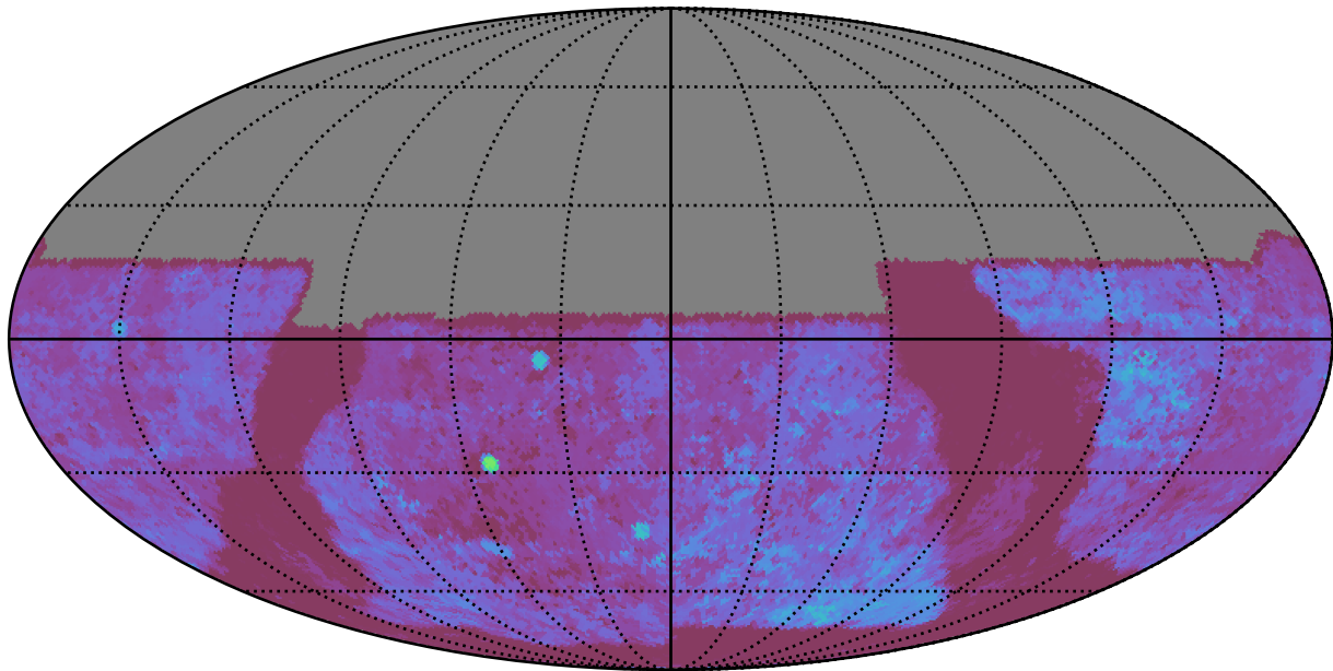
baseline_v2.1_10yrs All sky u band: Median Season Length
