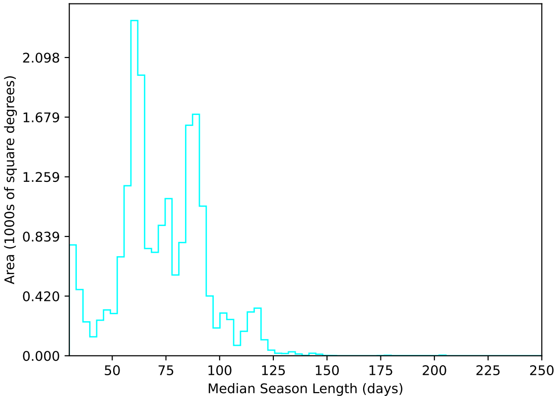
baseline_v2.1_10yrs All sky u band: Median Season Length
