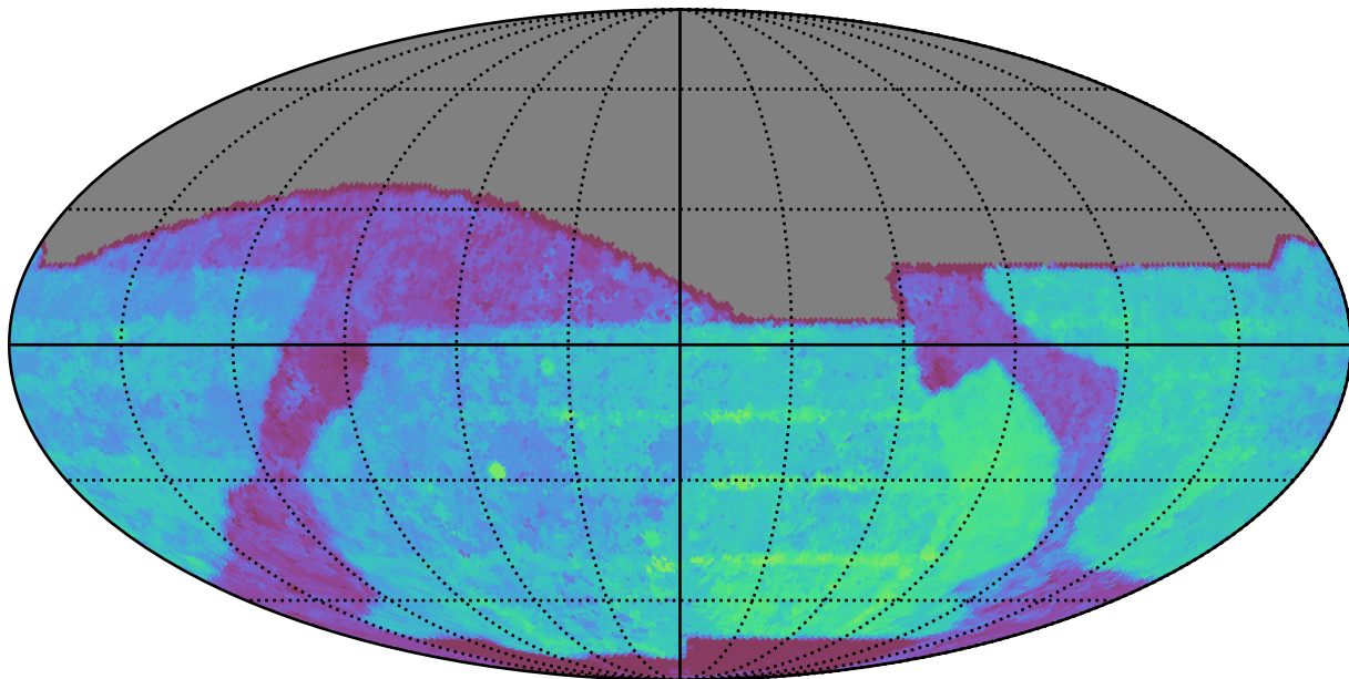
baseline_v2.1_10yrs All sky r band: Median Season Length
