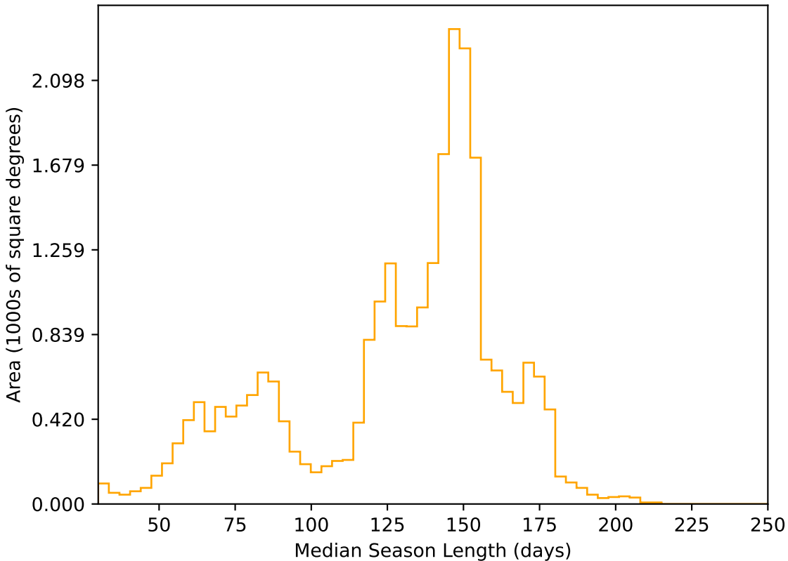
baseline_v2.1_10yrs All sky r band: Median Season Length
