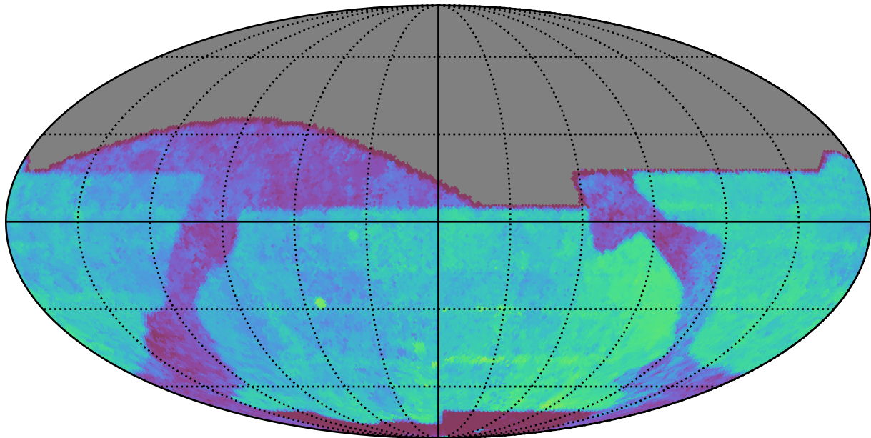
baseline_v2.1_10yrs All sky i band: Median Season Length
