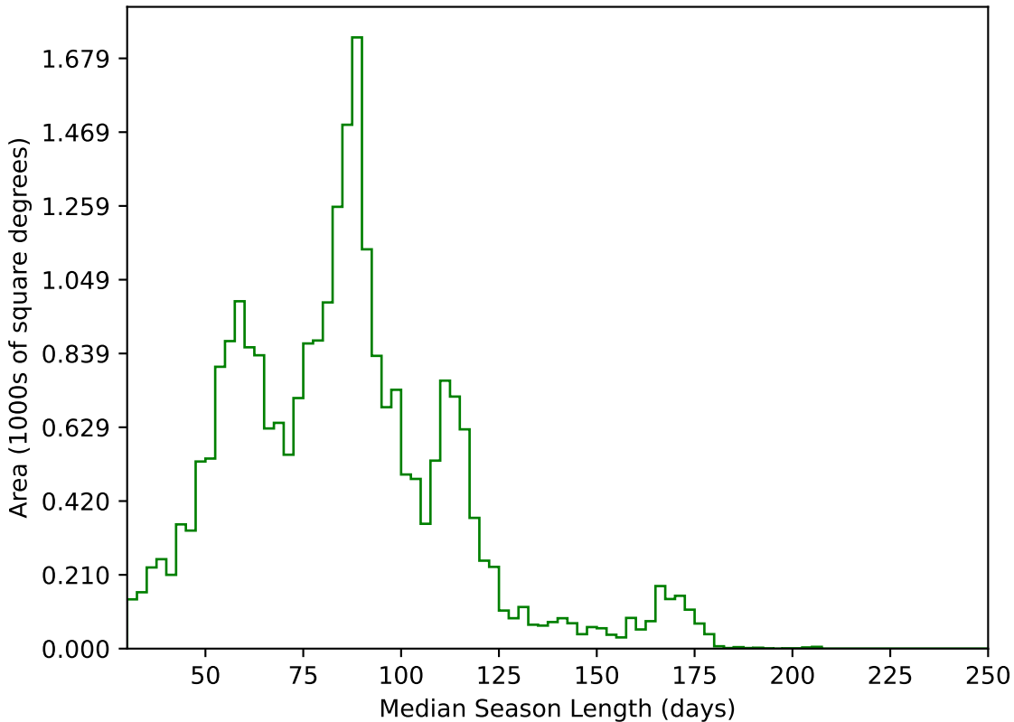
baseline_v2.1_10yrs All sky g band: Median Season Length
