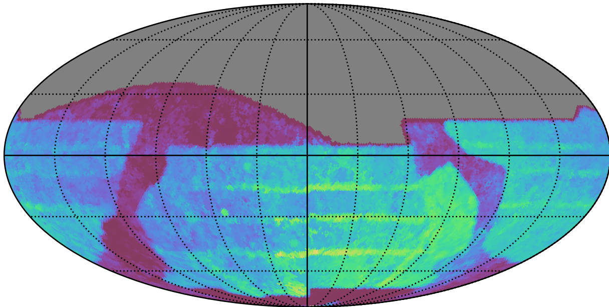
baseline_v2.1_10yrs All sky all bands: Median Season Length
