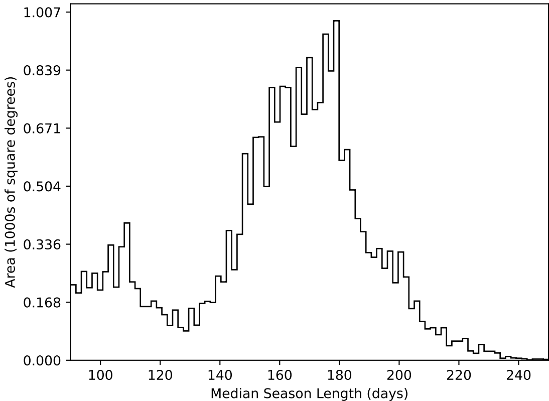
baseline_v2.1_10yrs All sky all bands: Median Season Length
