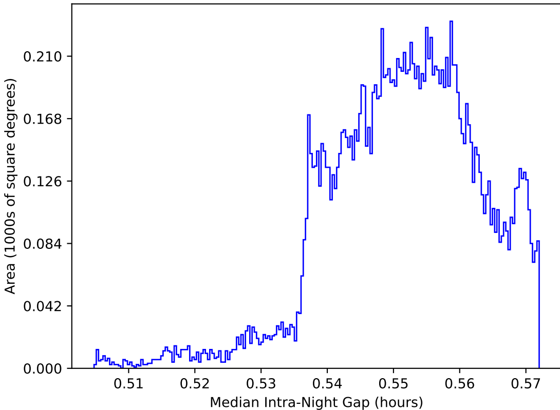
baseline_v2.1_10yrs WFD: Median Intra-Night Gap
