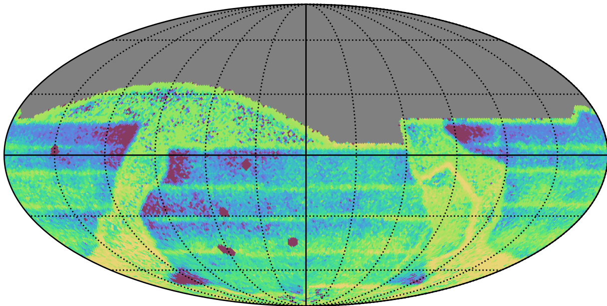
baseline_v2.1_10yrs All sky: Median Intra-Night Gap
