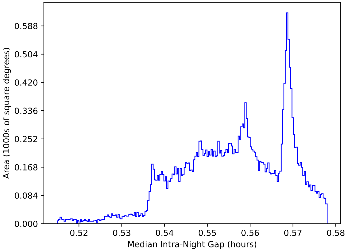
baseline_v2.1_10yrs All sky: Median Intra-Night Gap
