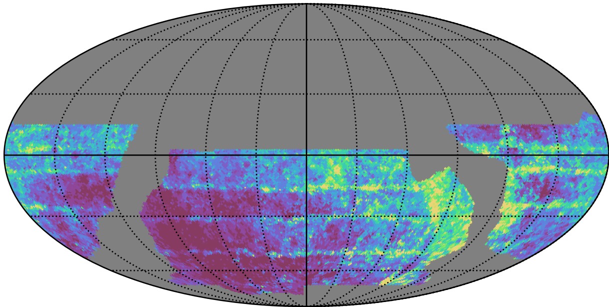
baseline_v2.1_10yrs WFD z band: Median Inter-Night Gap
