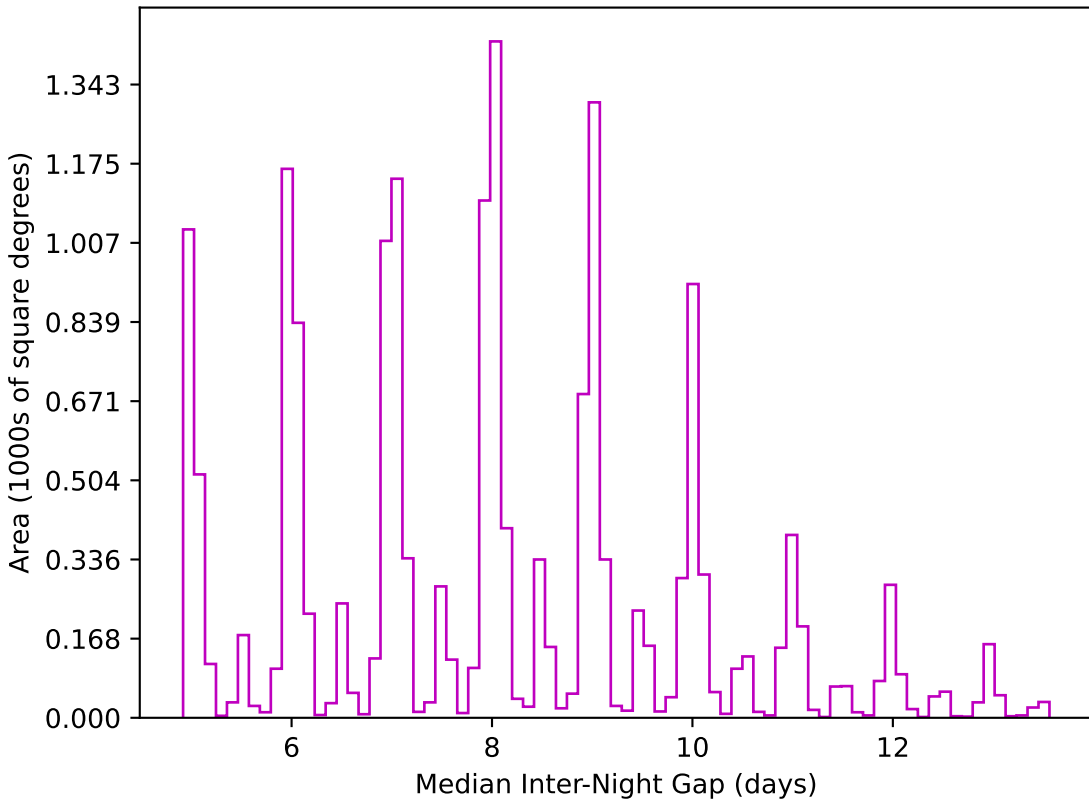
baseline_v2.1_10yrs WFD z band: Median Inter-Night Gap
