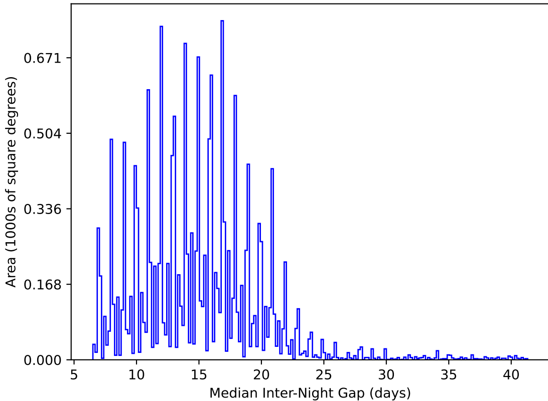
baseline_v2.1_10yrs WFD y band: Median Inter-Night Gap
