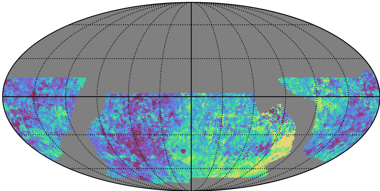
baseline_v2.1_10yrs WFD u band: Median Inter-Night Gap
