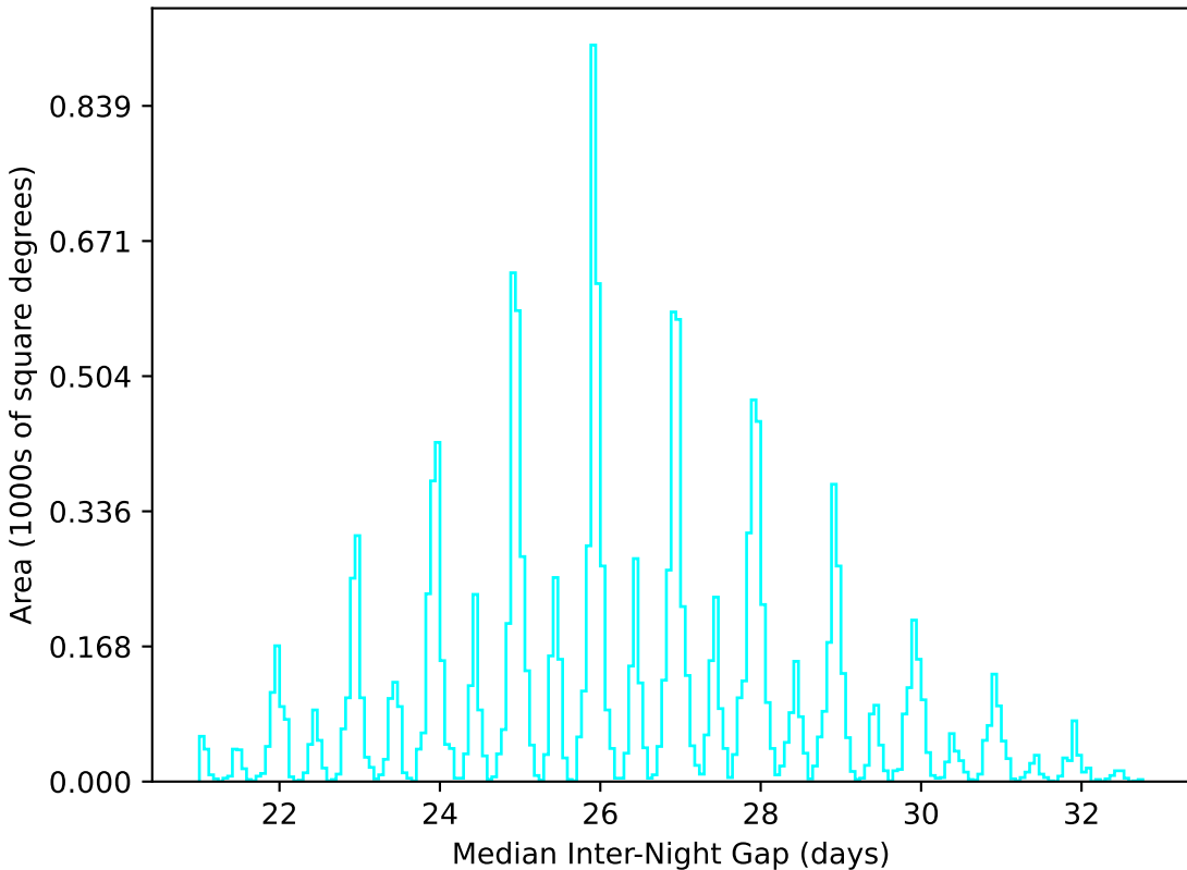
baseline_v2.1_10yrs WFD u band: Median Inter-Night Gap
