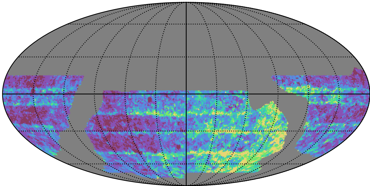
baseline_v2.1_10yrs WFD r band: Median Inter-Night Gap
