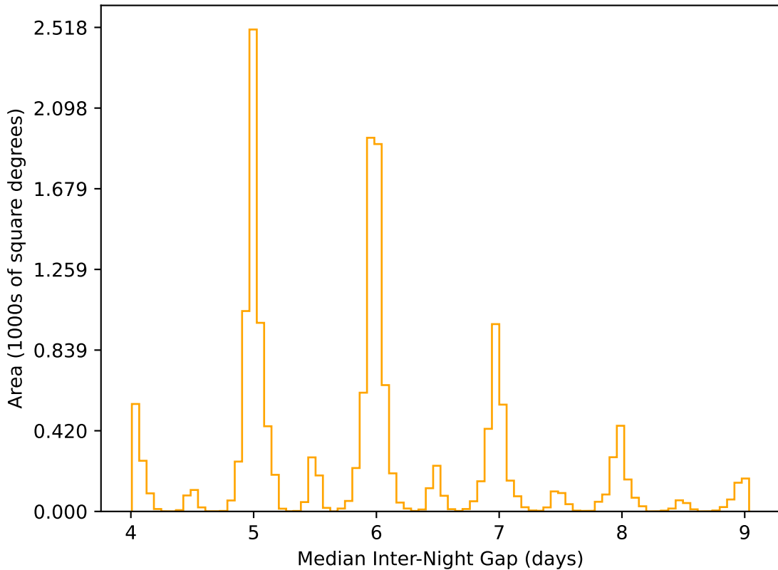
baseline_v2.1_10yrs WFD r band: Median Inter-Night Gap
