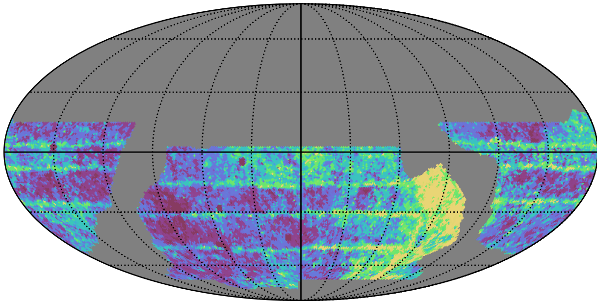
baseline_v2.1_10yrs WFD i band: Median Inter-Night Gap
