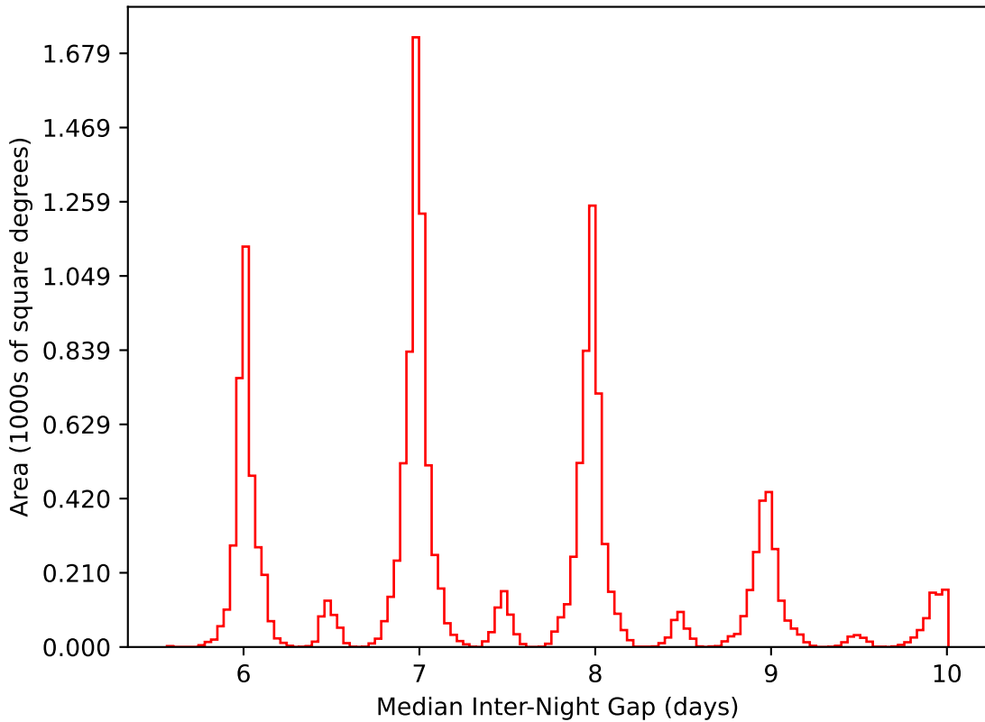
baseline_v2.1_10yrs WFD i band: Median Inter-Night Gap
