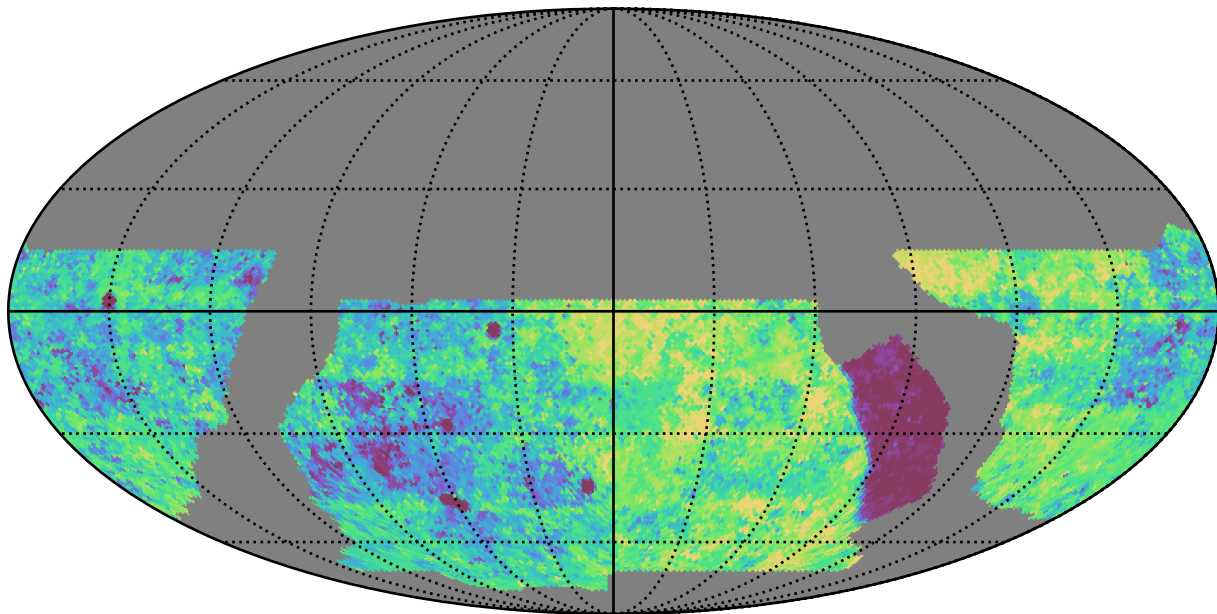
baseline_v2.1_10yrs WFD g band: Median Inter-Night Gap
