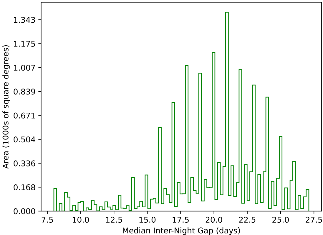
baseline_v2.1_10yrs WFD g band: Median Inter-Night Gap
