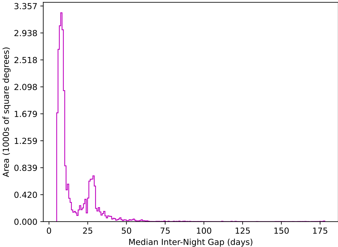
baseline_v2.1_10yrs All sky z band: Median Inter-Night Gap
