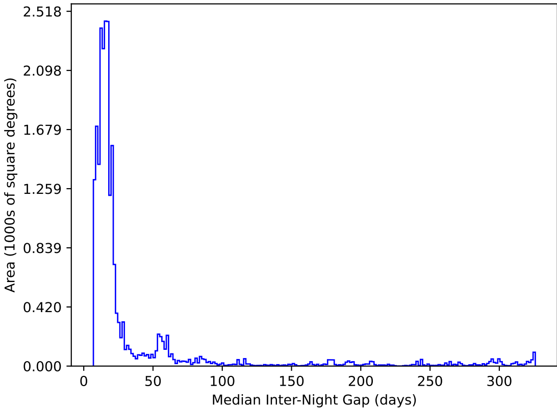
baseline_v2.1_10yrs All sky y band: Median Inter-Night Gap
