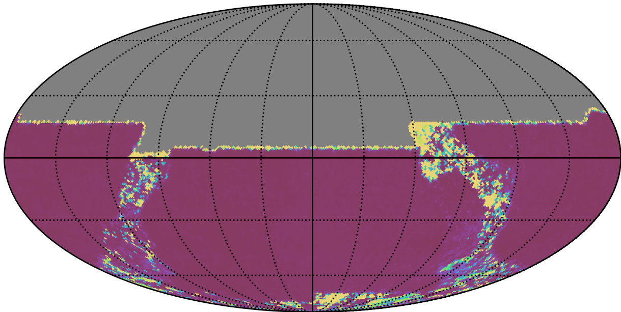
baseline_v2.1_10yrs All sky u band: Median Inter-Night Gap
