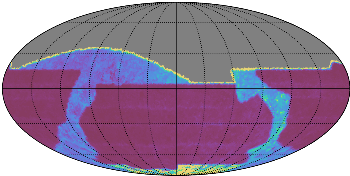
baseline_v2.1_10yrs All sky r band: Median Inter-Night Gap
