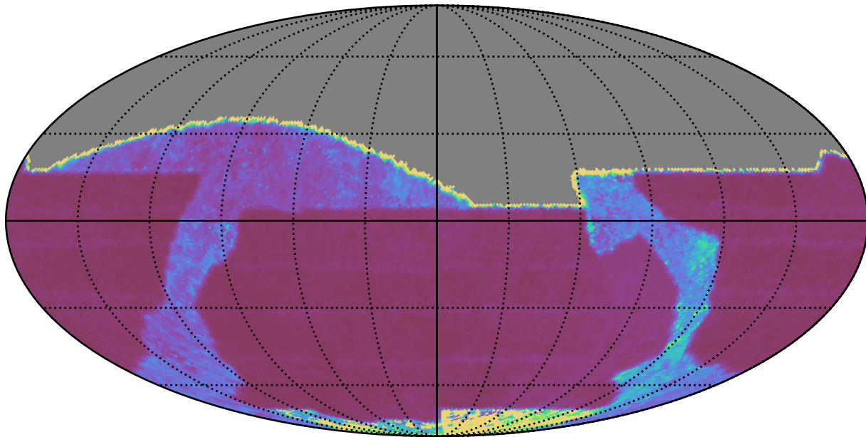
baseline_v2.1_10yrs All sky i band: Median Inter-Night Gap
