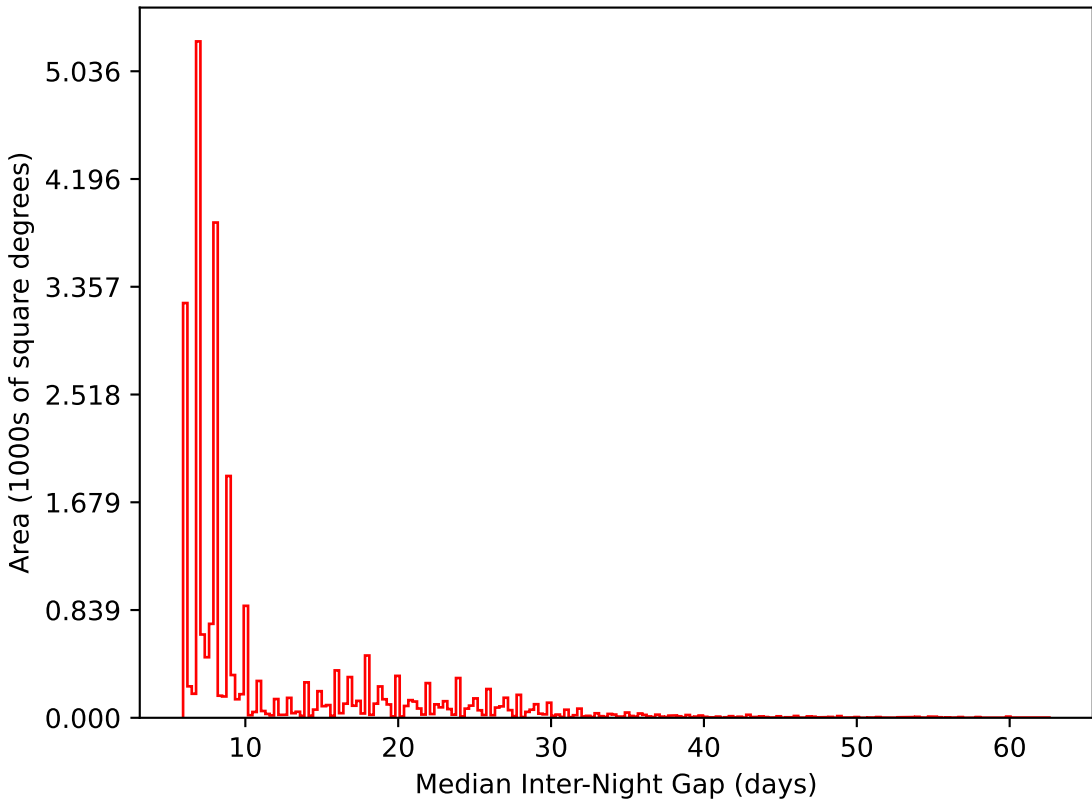
baseline_v2.1_10yrs All sky i band: Median Inter-Night Gap
