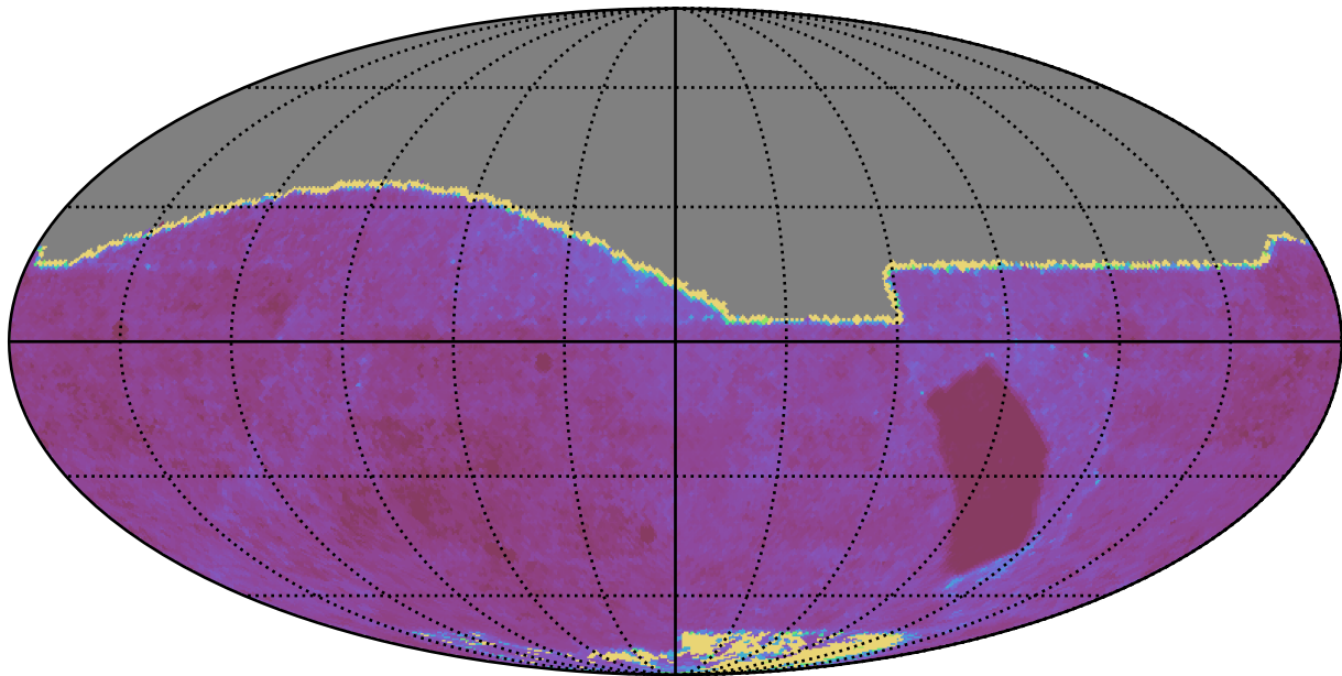
baseline_v2.1_10yrs All sky g band: Median Inter-Night Gap
