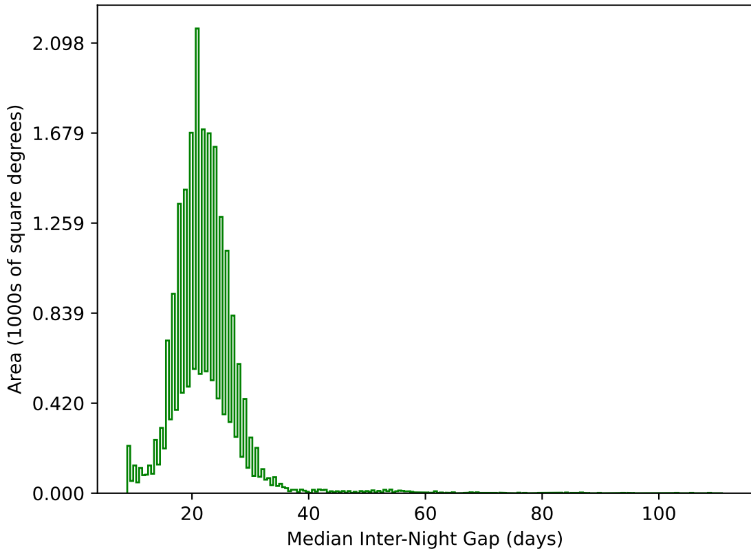
baseline_v2.1_10yrs All sky g band: Median Inter-Night Gap
