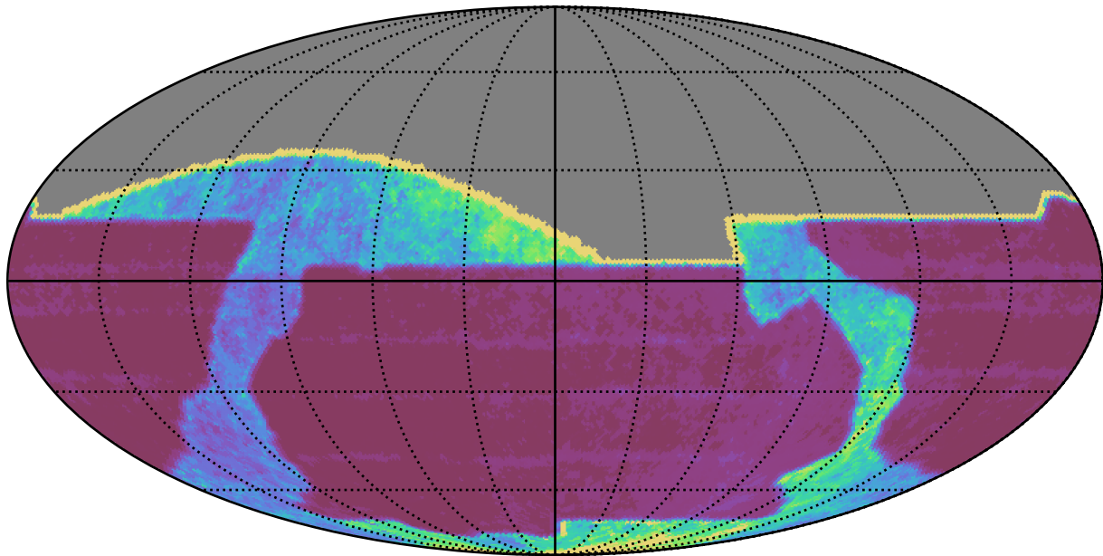
baseline_v2.1_10yrs All sky all bands: Median Inter-Night Gap
