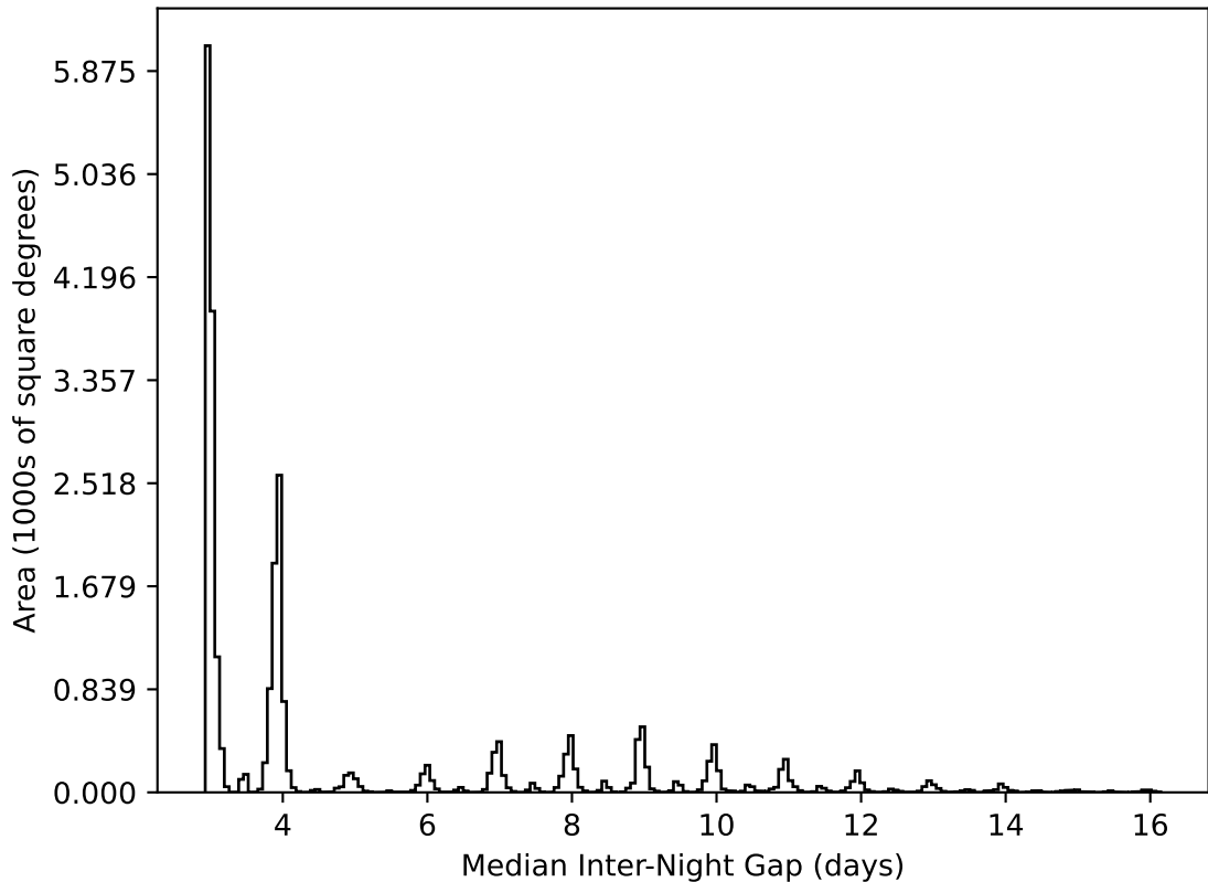
baseline_v2.1_10yrs All sky all bands: Median Inter-Night Gap
