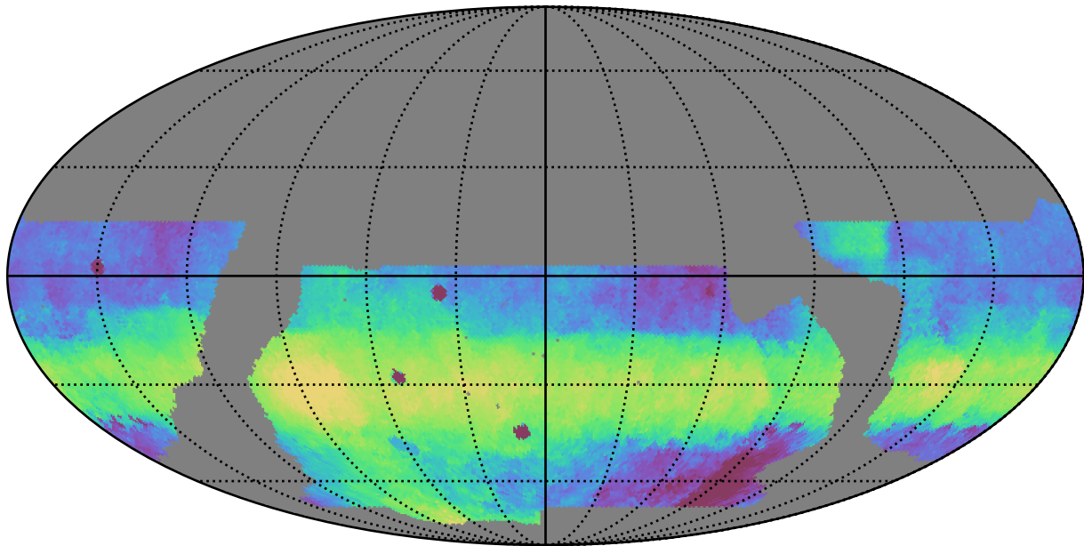
baseline_v2.1_10yrs WFD z band: Median HA
