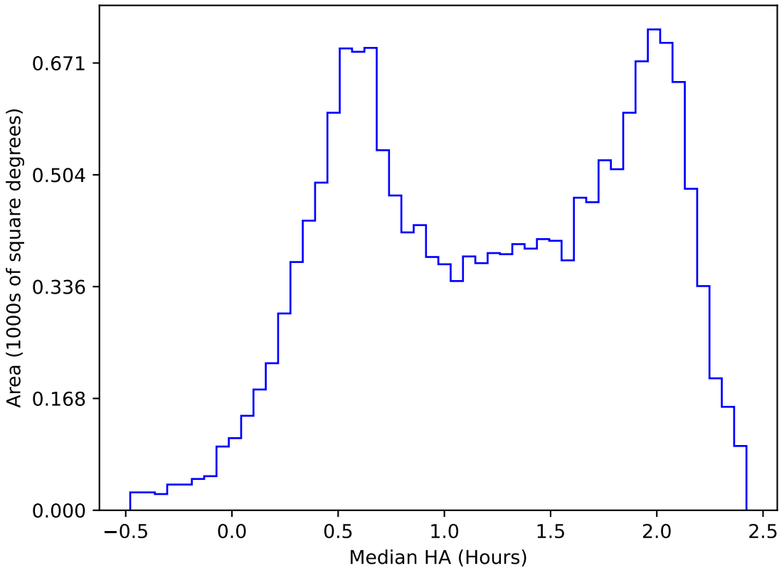
baseline_v2.1_10yrs WFD z band: Median HA
