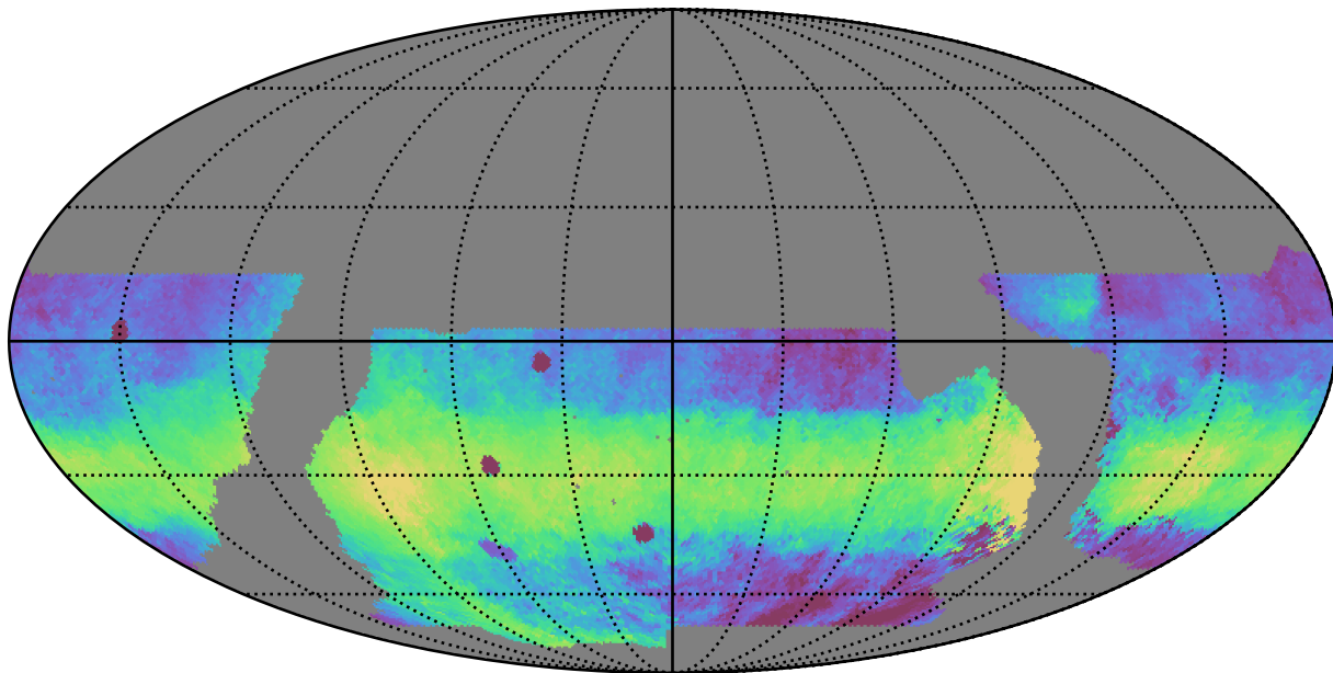
baseline_v2.1_10yrs WFD y band: Median HA
